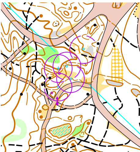
Station: 2 1:2 000
